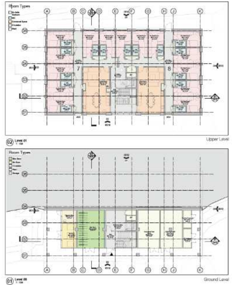
Residential Typology - Villas (Buildings 1, 6, 7, 8, 9, 13)
